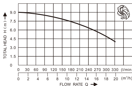
SPG 27502 DR
