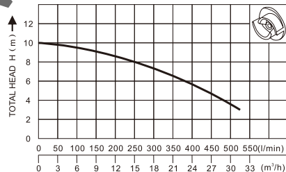
SPG 31502 CDR
