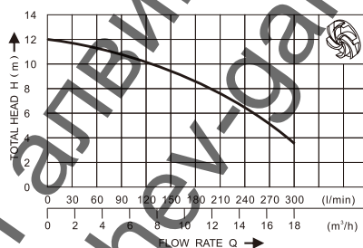
SPG 18502 CDR
