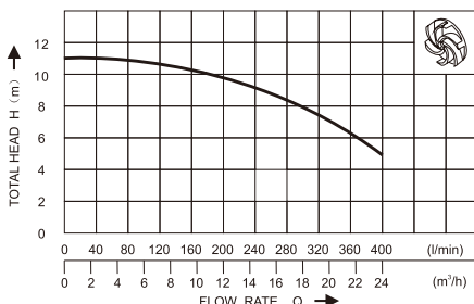
SPG 27502 DR
