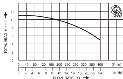
SPG 27502 DR
