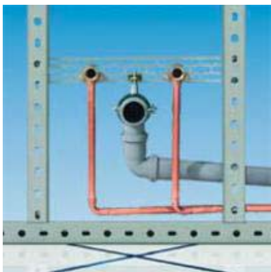
Wall-mounted installation: Wall-mounted installation with StaboFix® together with MÜPROMPC Channel Supports.
