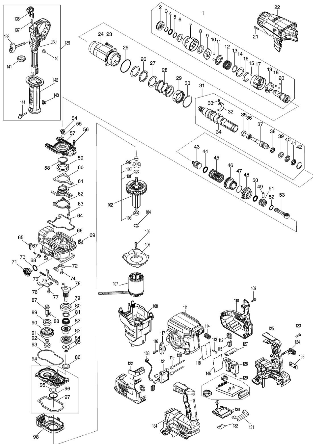
Model No.HR009G 30MM CRDLS COMBINATION HAMMER
