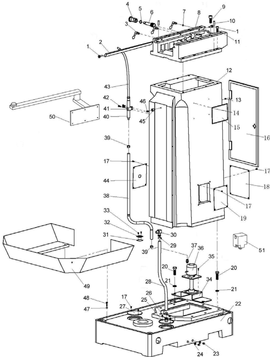
Abb. 1-1: Column and Base
