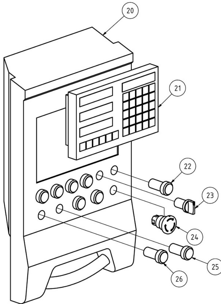
Abb. 1-25: Bedienpanel - Control panel
