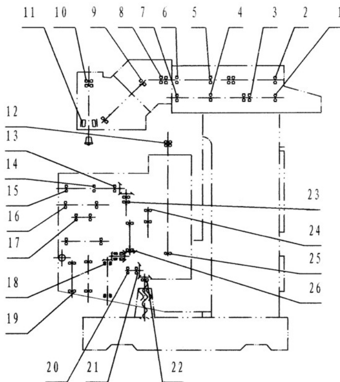
Abb.1-27: Overview bearings
