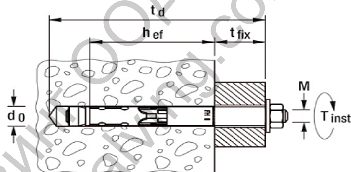
High performance anchor FH II - B
