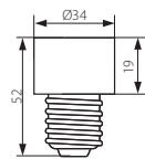
HLDR-E27/GU10
