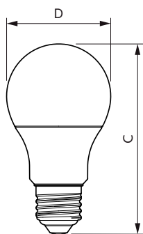
Bulb A60S+ 230V 8.5-60W 806lm 2700K E27
