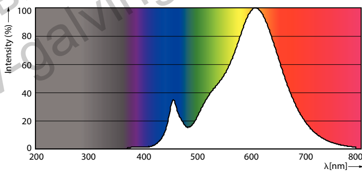
CorePro LEDbulb ND 19-150WA67E27 827FR
