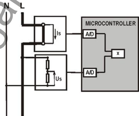
Fig. 7: Metering element
