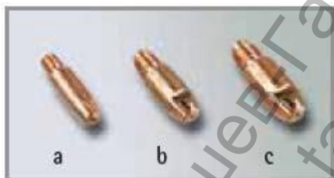
Ugello portacorrente - Contact tip - Buse
