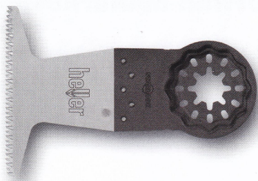
BIM wood precision-cutting saw, 50 x 65 mm Japanese toothing. Wood, plaster/render and soft plastics. Art.no.: 29539 0 & 29540 6
