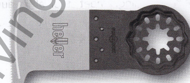
HCS wood & plastic saw, curved, 50 x 65 mm
