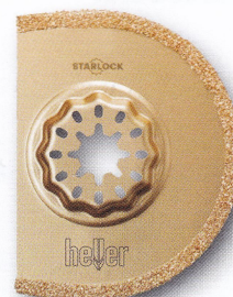
HCS hard materials saw, 75 x 2.2 mm For separating tile joints and slitting plaster/render and aerated concrete. Segmented, ideal for corners and edges. Art.no.: 29547 5
