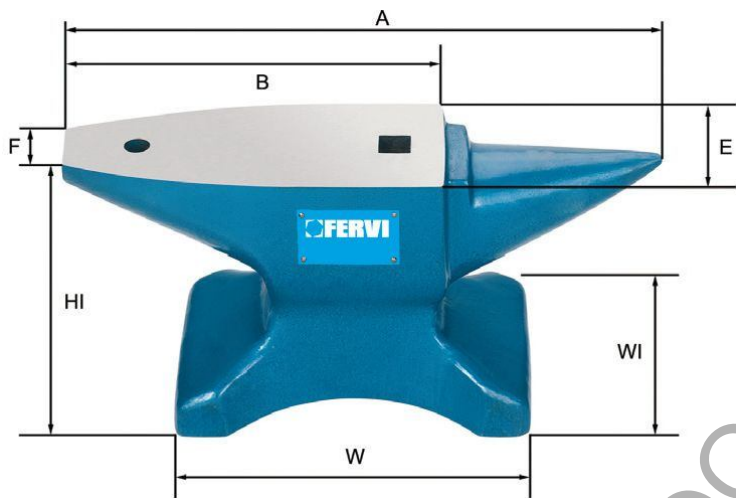
5 kg CAST IRON ANVIL
