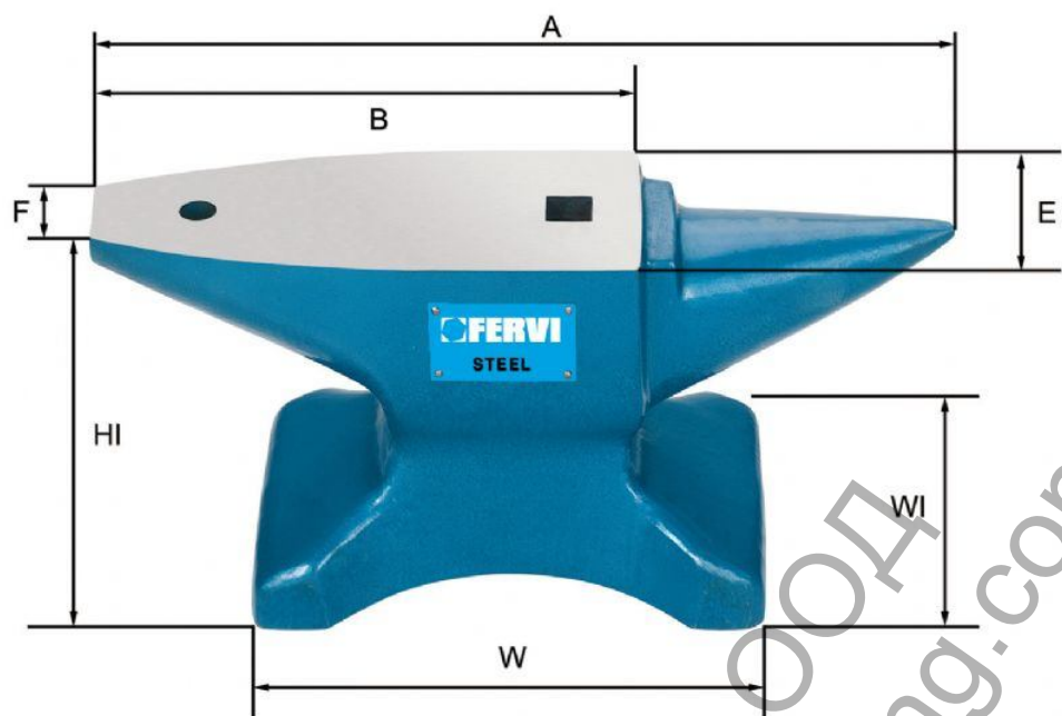
ART. 0157/100 C50 HARDENED STEEL ANVIL
